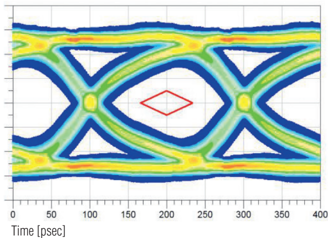
Eye Diagram at Receiver Output 5 GT/s
