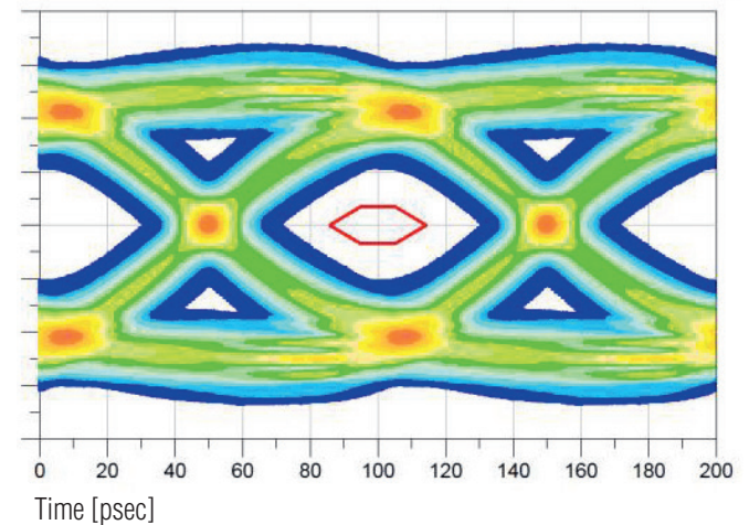
Eye Diagram at Receiver Output 10 GT/s
